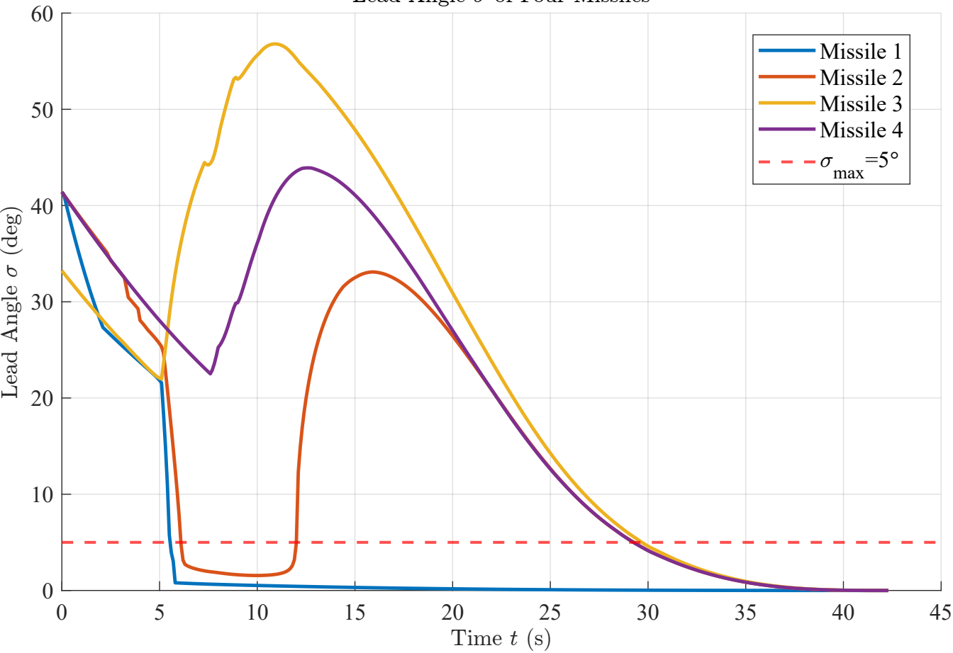
Lead Angle \sigma of Four Missiles
